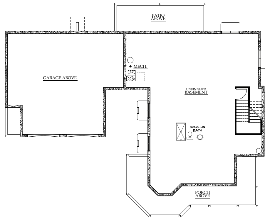
BASEMENT 1,505SF
