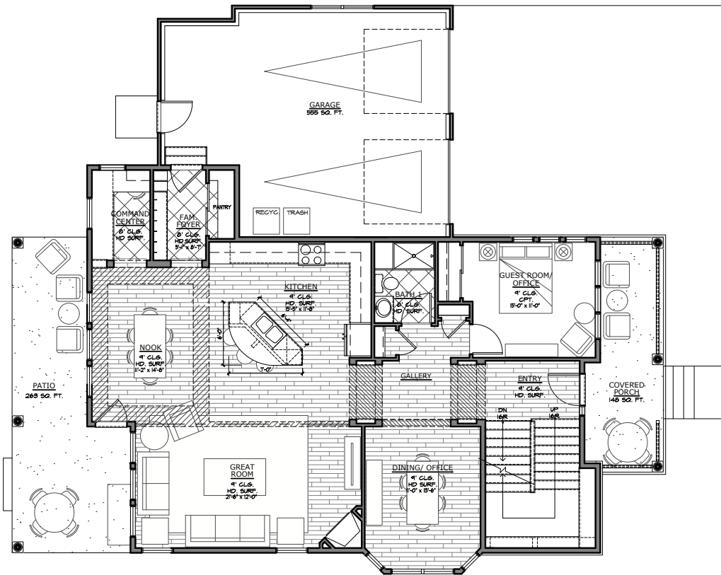
MAIN LEVEL
