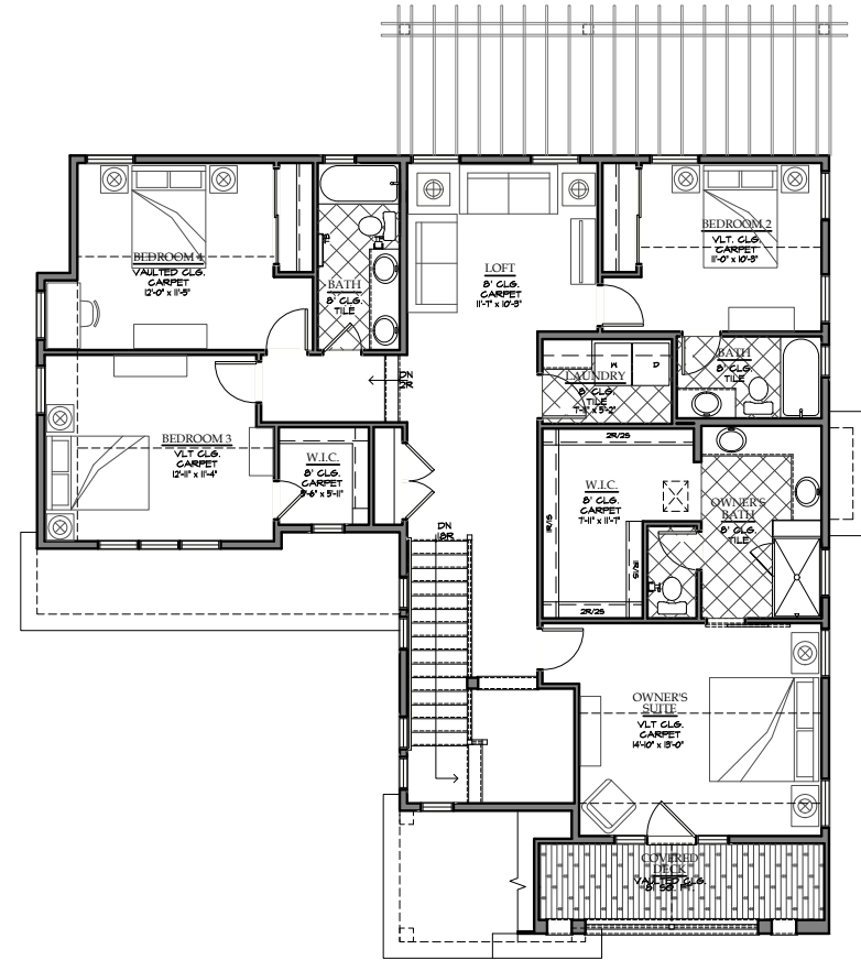
UPPER LEVEL
